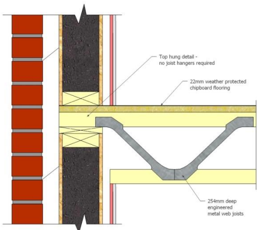
TOP HUNG METAL WEB JOIST
