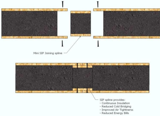
SIP SPLINE JOINT DETAIL
