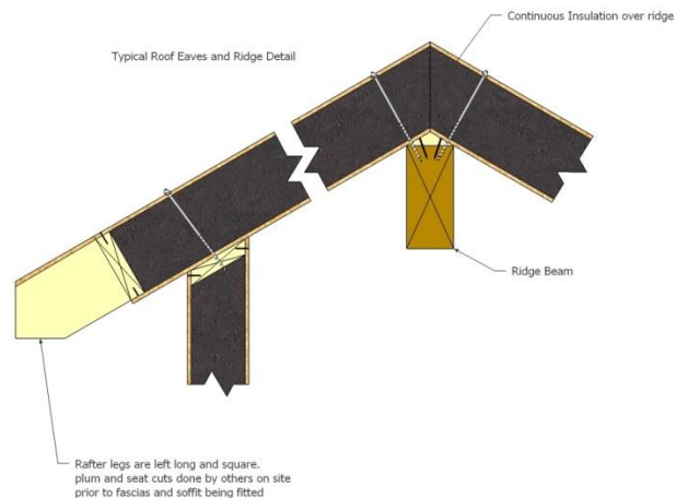
ROOF EAVES AND RIDGE
