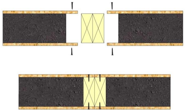
TIMBER SPLINE JOINT DETAIL
